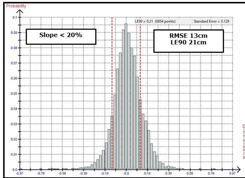
Figure 15. Histogram of the elevation differences between the WorldView-3 stereo satellite elevations for the 12.2km by 12km area and the 6854 elevation checkpoints with slopes less than 20% grade. The Guidelines for Digital Elevation Data of the US National Digital Elevation Program (NDEP) recommends that elevation checkpoints should be chosen in areas with slopes less than 20% grade. RMSE 13cm, LE90 21cm.
