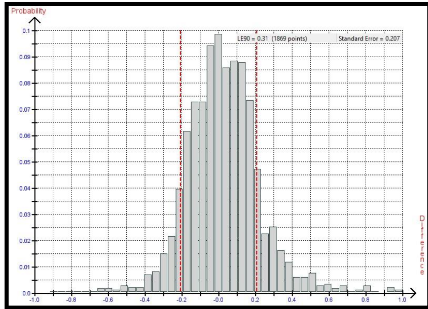
Figure 16. Histogram of the elevation differences between the WorldView-2 stereo satellite elevations for the 12.2km by 12km area and the 1,869 elevation checkpoints with slopes between 20% and 100% grade. RMSE 21cm, LE90 31cm.
