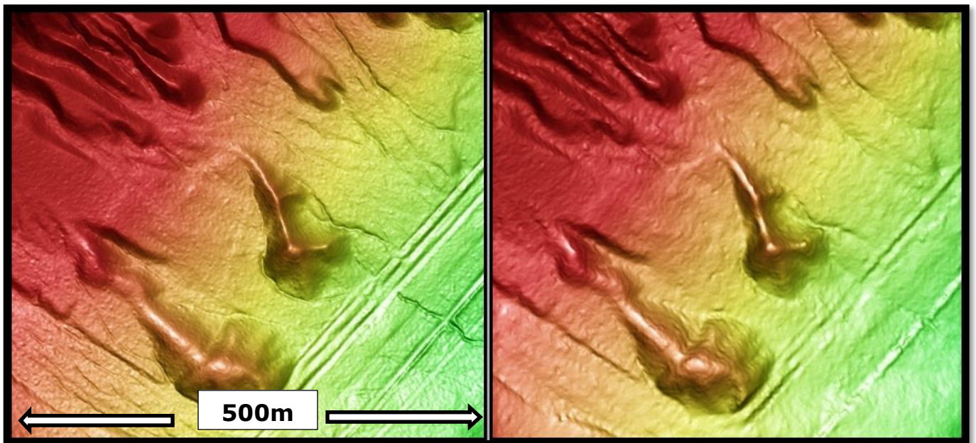
Figure 12. Comparison of the elevation grids between the LiDAR on the left and the stereo WorldView-2 on the right. This is for a 500m wide area. More topographic detail is visible on the LiDAR at this scale.
