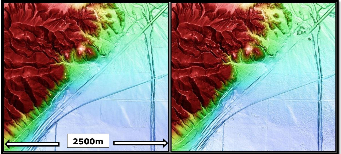
Figure 11. Comparison of the elevation grids between the LiDAR on the left and the stereo WorldView-2 on the right. This is for a 2,500m wide area. Minor differences between the elevation grids are visible at this scale.
