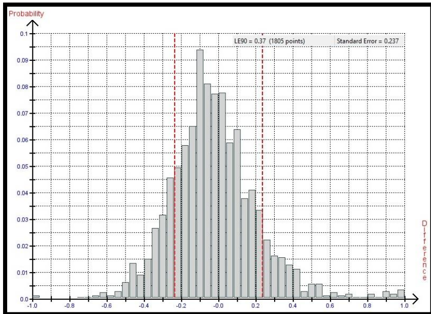
Figure 16. Histogram of the elevation differences between the WorldView-2 stereo satellite elevations for the 14.5km by 12km area and the 1805 elevation checkpoints with slopes between 20% and 100% grade. RMSE 24cm, LE90 37cm.
