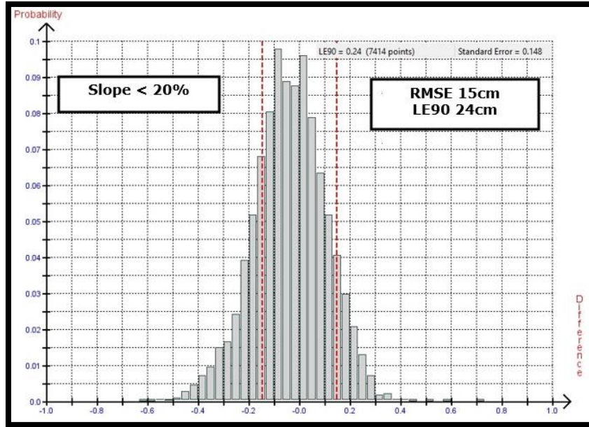
Figure 15. Histogram of the elevation differences between the WorldView-2 stereo satellite elevations for the 14.5km by 12km area and the 7,414 elevation checkpoints with slopes less than 20% grade. The Guidelines for Digital Elevation Data of the US National Digital Elevation Program (NDEP) recommends that elevation checkpoints should be chosen in areas with slopes less than 20% grade. RMSE 15cm, LE90 24cm.
