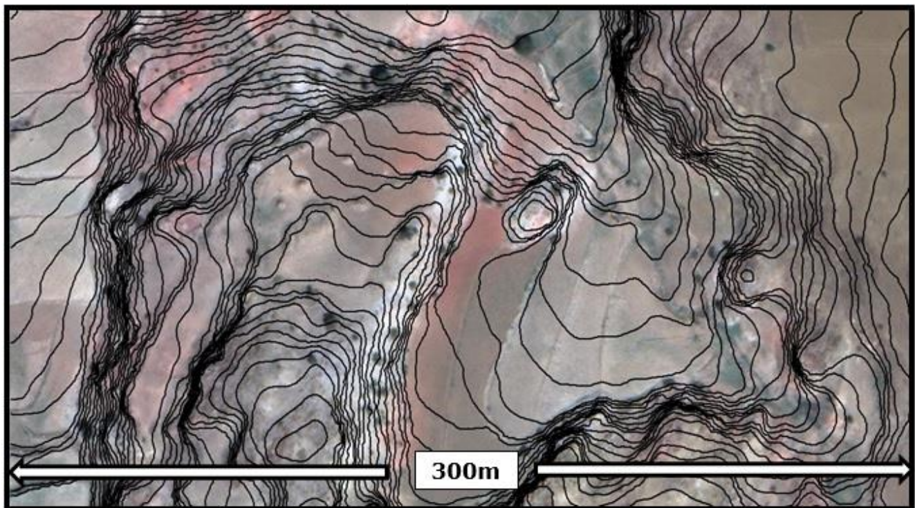
Figure 1. WorldView-3 color image with 50cm contours from the PhotoSat WorldView-3 survey of the Eritrea test area.
