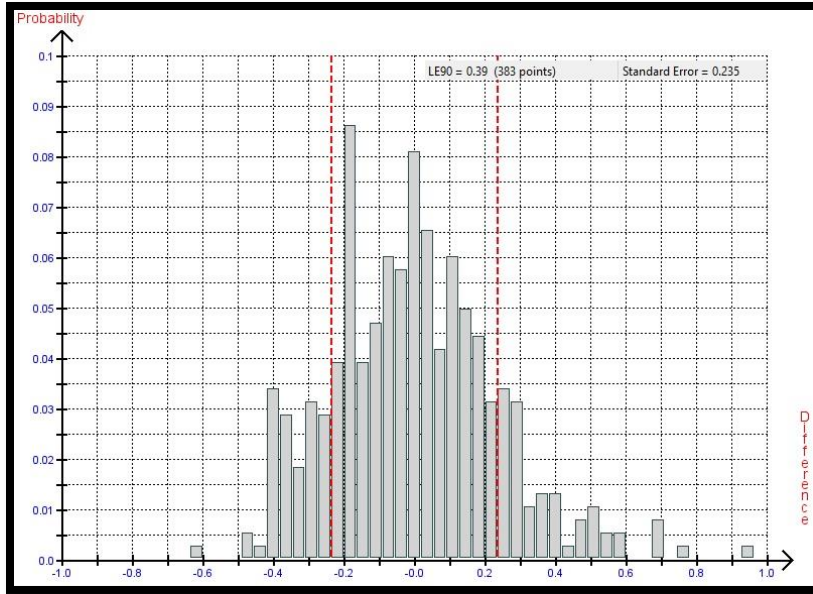
Figure 13. Histogram of the elevation differences between the WorldView-3 stereo satellite elevations for the 18 km by 11 km area and the 383 elevation checkpoints with slopes between 20% and 100% grade. RMSE 24cm, LE90 39cm.
