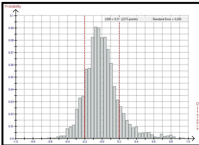
Figure 12. Histogram of the elevation differences between the WorldView-3 stereo satellite elevations for the 18 km by 11km area and all 2,273 elevation checkpoints. RMSE 20cm, LE90 31cm.
