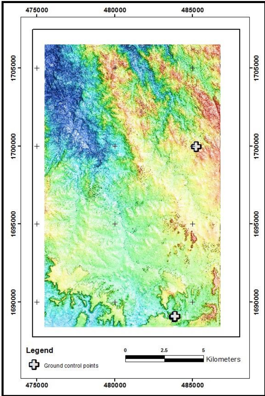
Figure 7. Stereo WorldView-3 elevation image created from the 1m PhotoSat Asmara, Eritrea satellite survey grid. The figure shows the locations of the two ground control points.
