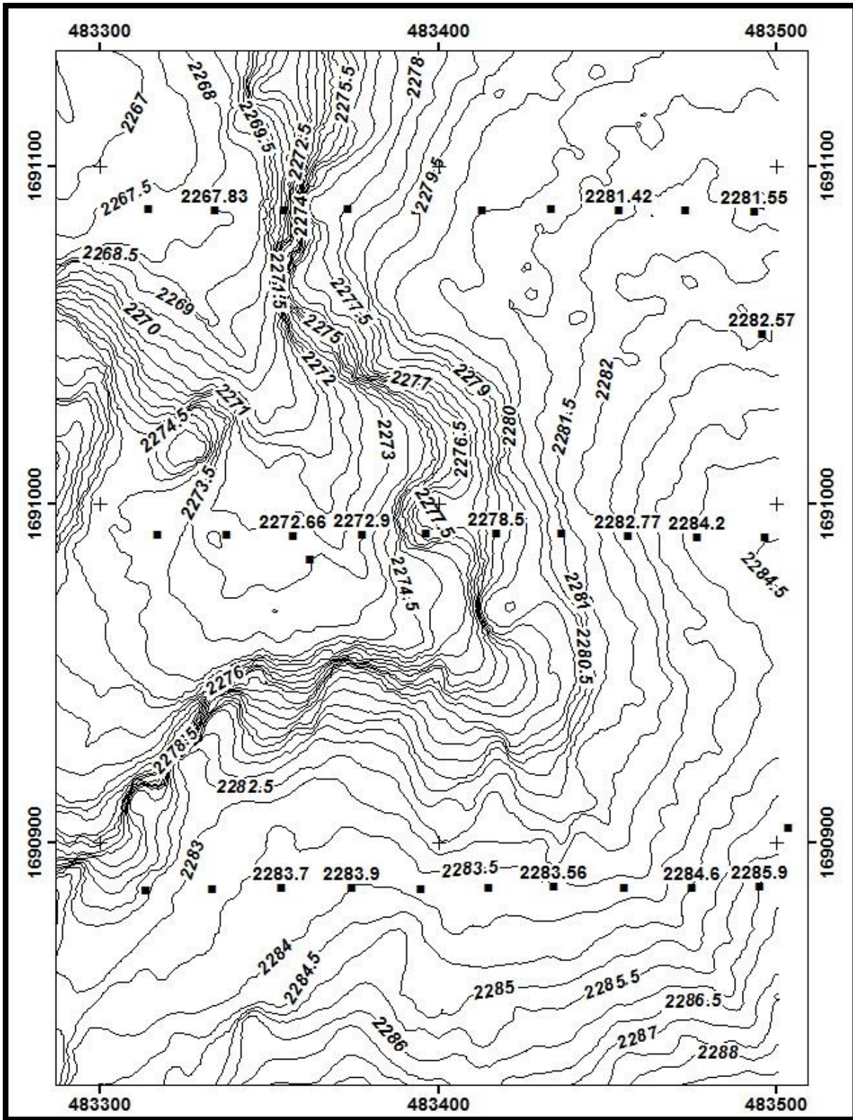
Figure 14. 50cm contours from the stereo WorldView-3 elevation survey comparing the contour elevations to some of the elevation checkpoints.
