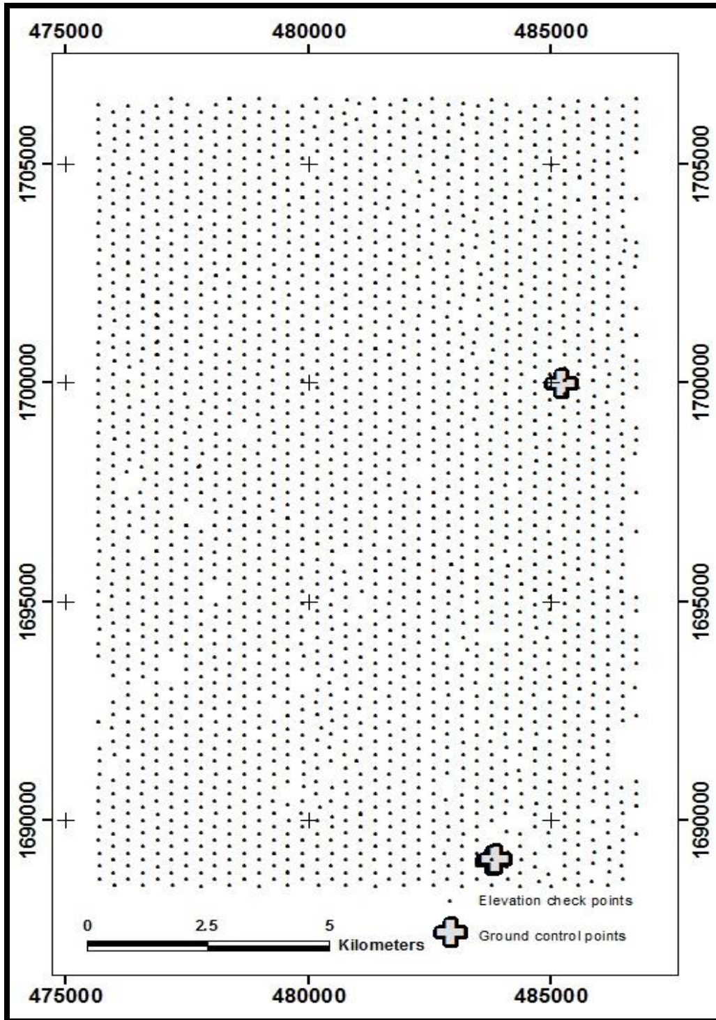
Figure 9. Area of the 18km by 11km Eritrea Stereo WorldView-3 1m elevation grid showing the two ground control points and the 1,803 gravity survey stations used as elevation checkpoints to determine the accuracy of the stereo satellite survey.
