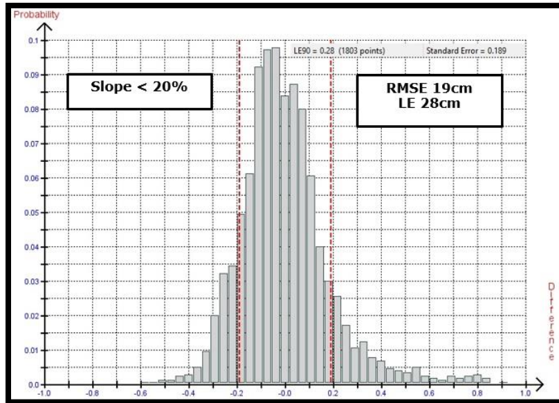
Figure 11. Histogram of the elevation differences between the WorldView-3 stereo satellite elevations for the 18km by 11km area and the 1,803 elevation checkpoints with slopes less than 20% grade. The Guidelines for Digital Elevation Data of the US National Digital Elevation Program (NDEP) recommends that elevation checkpoints should be chosen in areas with slopes less than 20% grade. RMSE 19cm, LE90 28cm.
