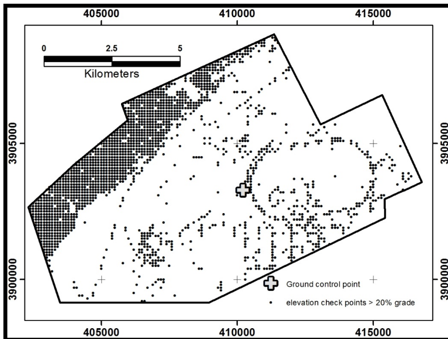
Figure 14. Elevation checkpoints for areas with slopes of greater than 20% grade.
