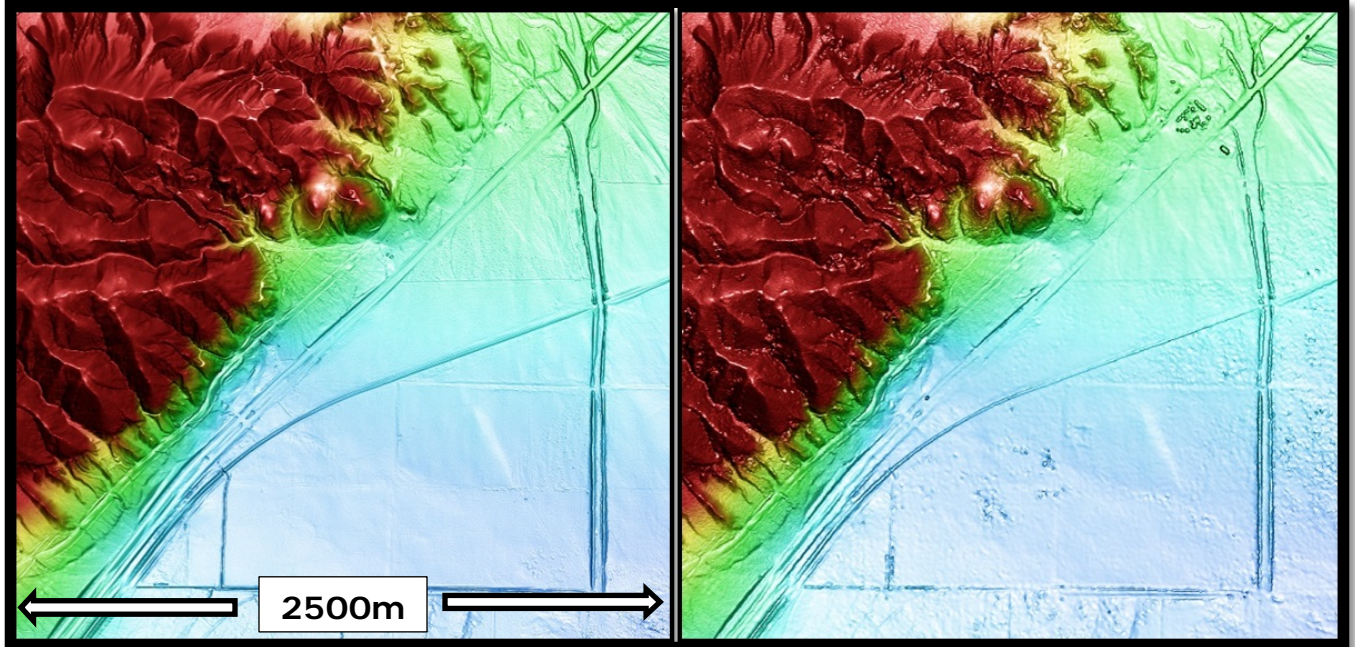
Figure 11. Comparison of the elevation grids between the LiDAR on the left and the stereo Kompsat-3A on the right. This is for a 2,500m wide area. Minor differences between the elevation grids are visible at this scale.
