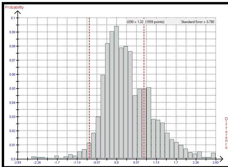
Figure 16. Histogram of the elevation differences between the Kompsat-3A stereo satellite elevations for the 14.5km by 9.9km area and the 1,959 elevation checkpoints with slopes between 20% and 100% grade. RMSE 78cm, LE90 1.32m.
