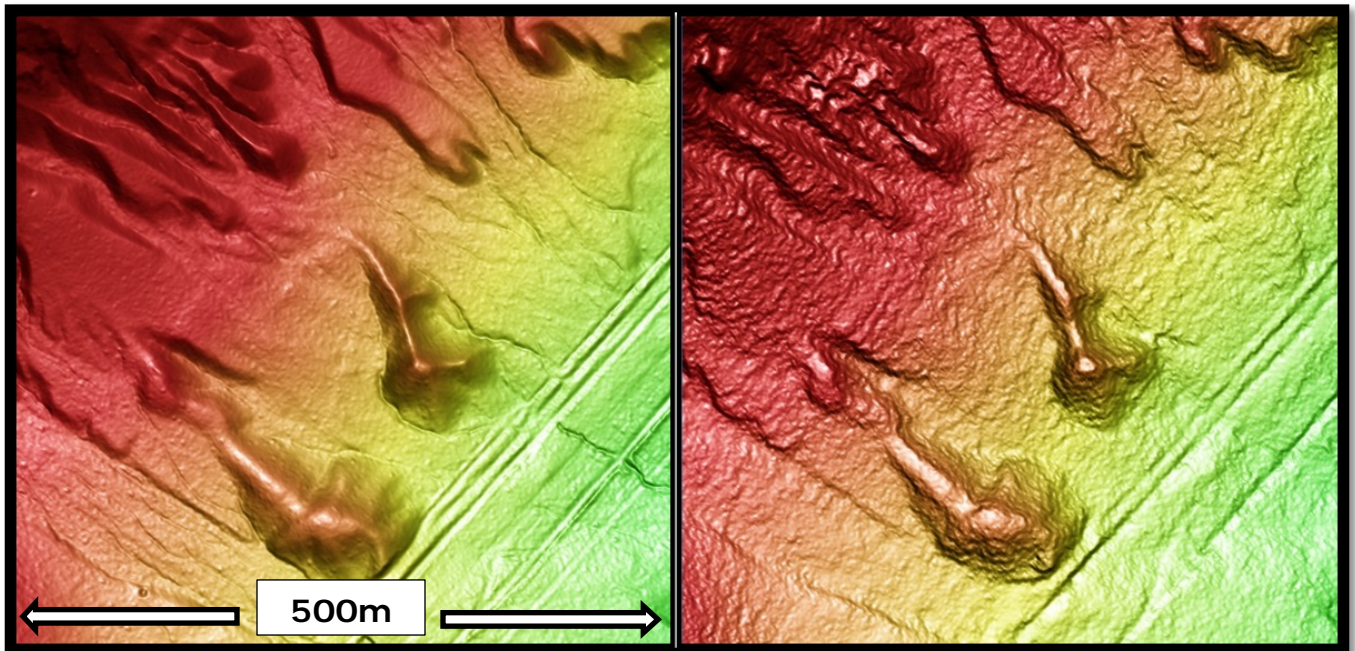
Figure 12. Comparison of the elevation grids between the LiDAR on the left and the stereo Kompsat-3A on the right. This is for a 500m wide area. More topographic detail is visible on the LiDAR at this scale.
