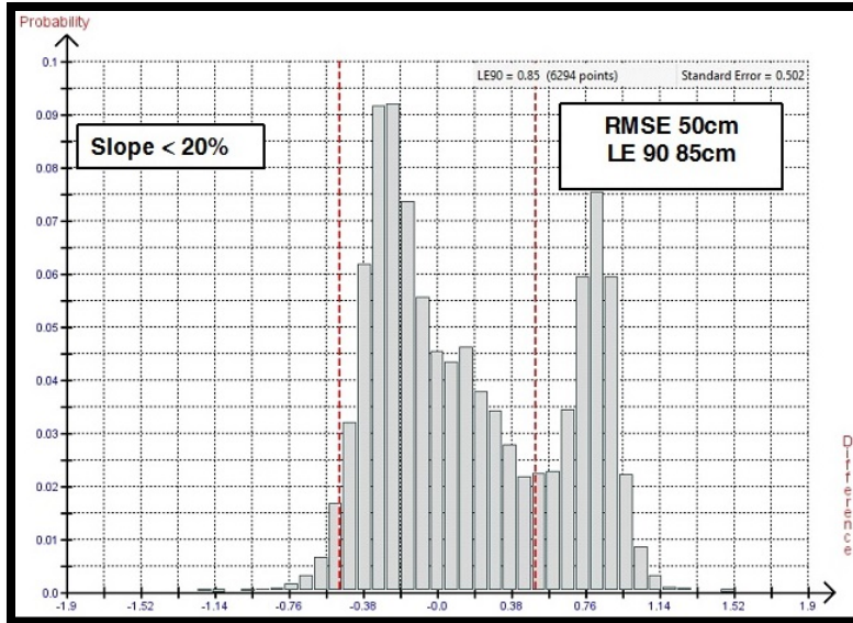
Figure 15. Histogram of the elevation differences between the Kompsat-3A stereo satellite elevations for the 14.5km by 9.9km area and the 6,294 elevation checkpoints with slopes less than 20% grade. The Guidelines for Digital Elevation Data of the US National Digital Elevation Program (NDEP) recommends that elevation checkpoints should be chosen in areas with slopes less than 20% grade. RMSE 50cm, LE90 85cm.
