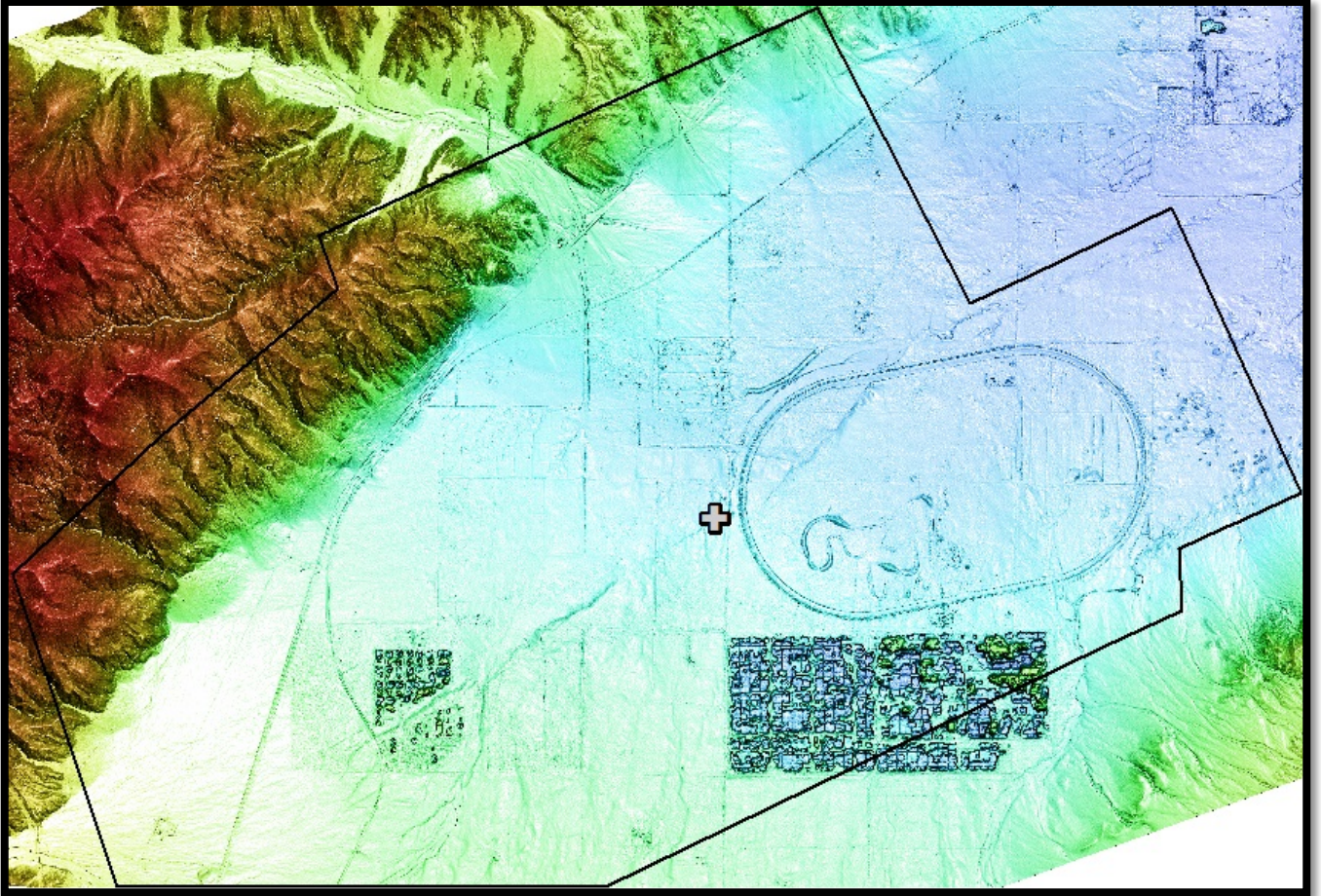
Figure 10. Stereo Kompsat-3A elevation image covering the area of the LiDAR image in Figure 3. This elevation grid has an elevation point every meter. At this scale, the LiDAR and Kompsat-3A images are identical. Low elevations are blue and high elevations are red.
