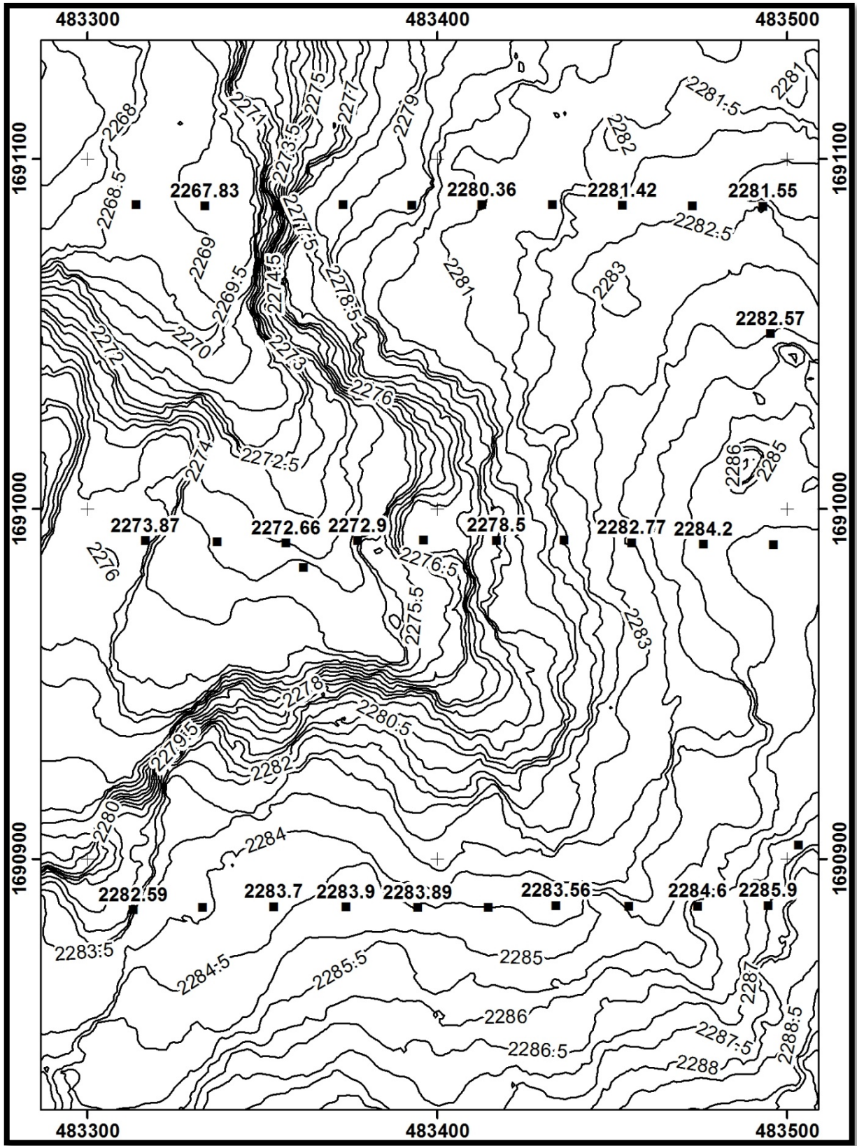
Figure 14. 50cm contours from the stereo Kompsat-3A elevation survey comparing the contour elevations to some of the elevation checkpoints.
