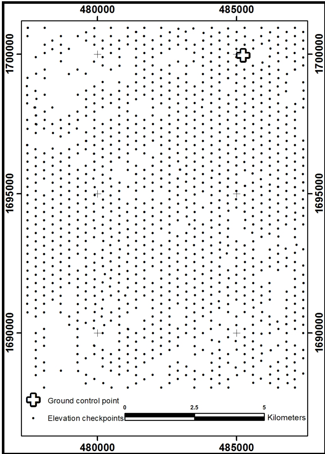
Figure 9. Area of the 13km by 10km Eritrea Stereo Kompsat-3A 1m elevation grid showing the ground control point and the 1,406 gravity survey stations used as elevation checkpoints to determine the accuracy of the stereo satellite survey.
