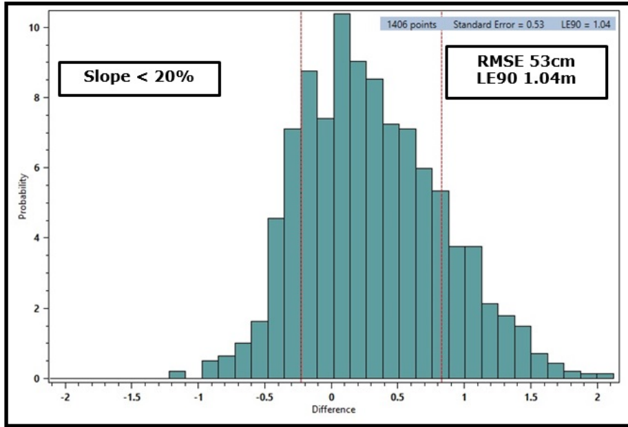
Figure 11. Histogram of the elevation differences between the Kompsat-3A stereo satellite elevations for the 13km by 10km area and the 1,406 elevation checkpoints with slopes less than 20% grade. The Guidelines for Digital Elevation Data of the US National Digital Elevation Program (NDEP) recommends that elevation checkpoints should be chosen in areas with slopes less than 20% grade. RMSE 53cm, LE90 1.04m.
