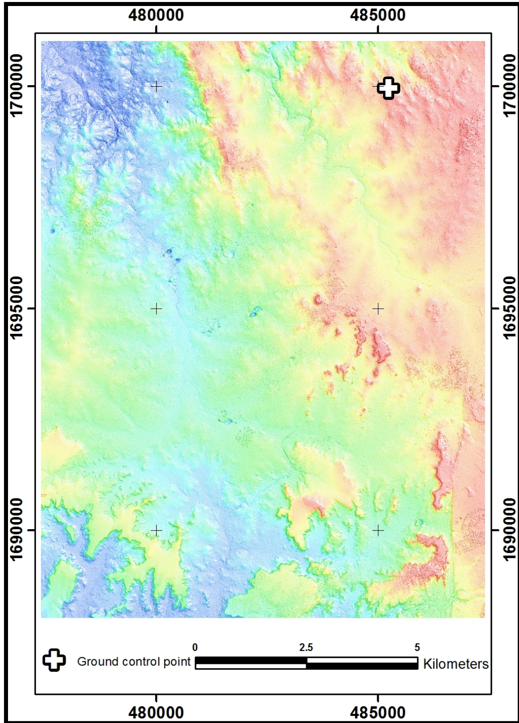
Figure 7. Stereo Kompsat-3A elevation image created from the 1m PhotoSat Asmara, Eritrea satellite survey grid. The figure shows the locations the ground control point.
