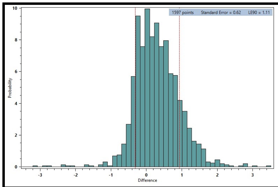
Figure 12. Histogram of the elevation differences between the Kompsat-3A stereo satellite elevations for the 13 km by 10km area and all 1,597 elevation checkpoints. RMSE 62cm, LE90 1.11m.
