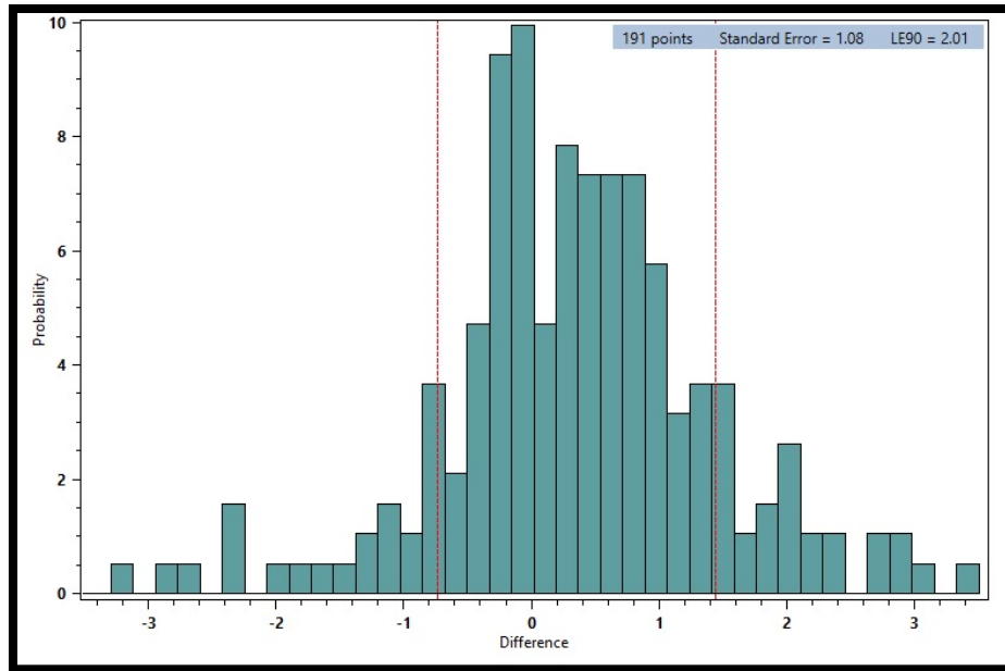
Figure 13. Histogram of the elevation differences between the Kompsat-3A satellite elevations for the 13 km by 10 km area and the 191 elevation checkpoints with slopes between 20% and 100% grade. RMSE 1.08m, LE90 2.01m.
